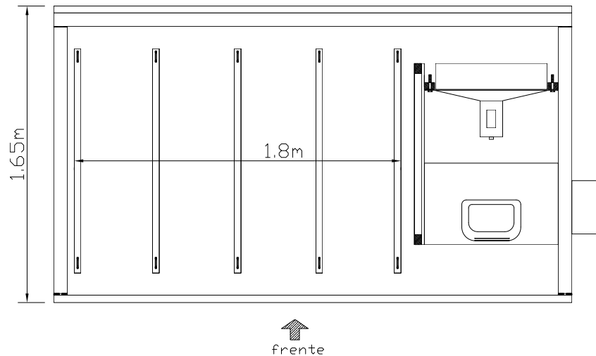
VISTA SUPERIOR MF 500-6S (sin techo)
