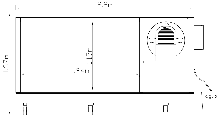
VISTA FRONTAL MF 500-6S (sin puerta)
